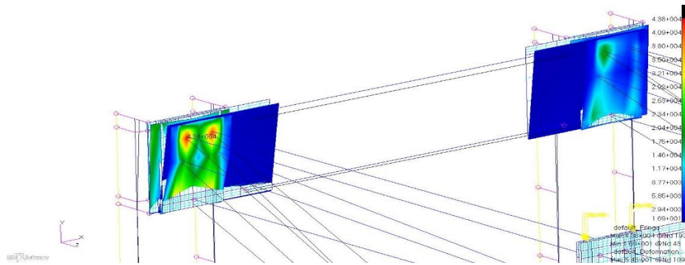
Figure 6. Maximal Stresses in the Plates
