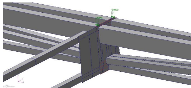
Figure 5. Details of Bridge Joint Model
